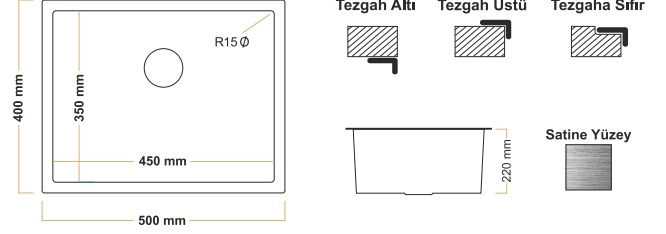
350x450 mm \varnothing R10/R15/R20 SH3545
