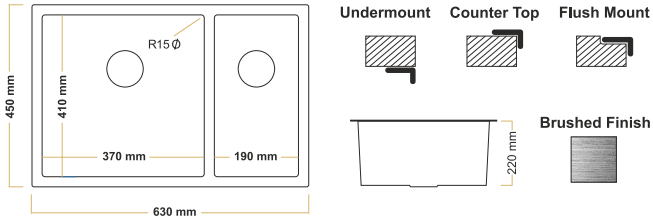
450x630 mm Ø R10/R15/R20 SH4563
