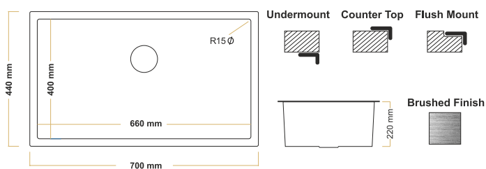
400x660 mm \varnothing R10/R15/R20 SH4066
