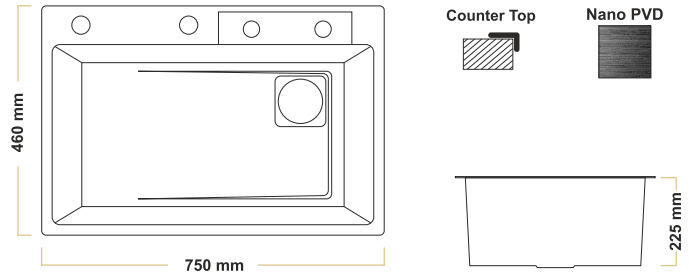
460x750 mm SH4675
