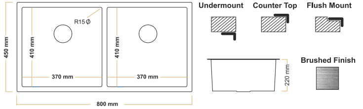
450x800 mm Ø R10/R15/R20 SH4580
