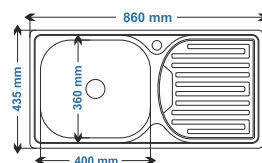
435x860 mm (With Overflow)
