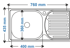
435x760 mm (With Overflow)
